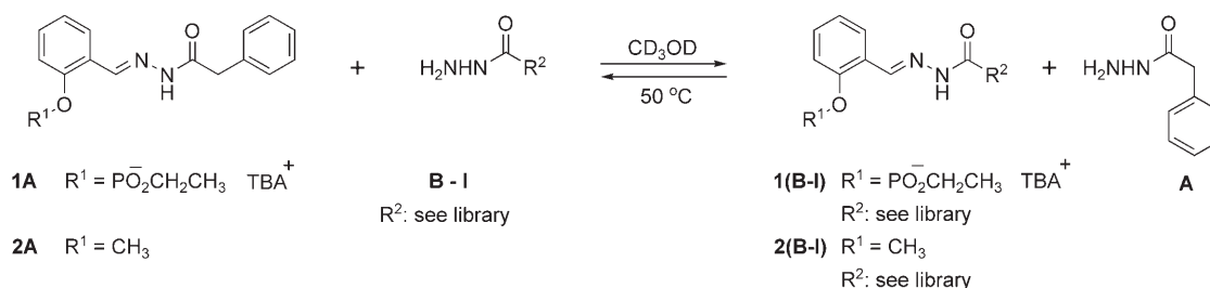
Scheme 2. Competition experiments. All experiments were performed using scaffold 1 (or 2 , 5 mM), hydrazide A and either one of the hydrazides B–I in a 1:5:5 ratio in CD 3 OD at 50 °C.
