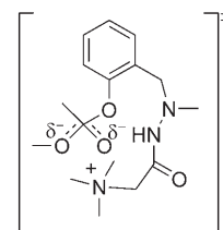
Figure 3. Stabilization of the transition state during the methanolysis of 3B .
