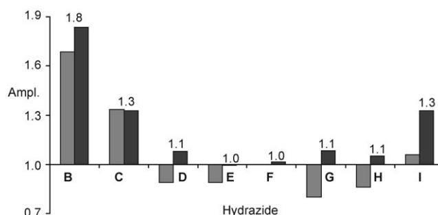
Figure 1. Observed amplification for each hydrazide in reference to hydrazide A obtained either from 1 H– 13 C HSQC-spectra (light gray bars) or from separate mixing experiments (dark gray bars).
